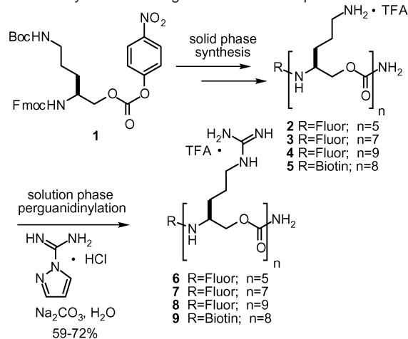
Scheme 1. Synthesis of Oligocarbamate Transporters a
